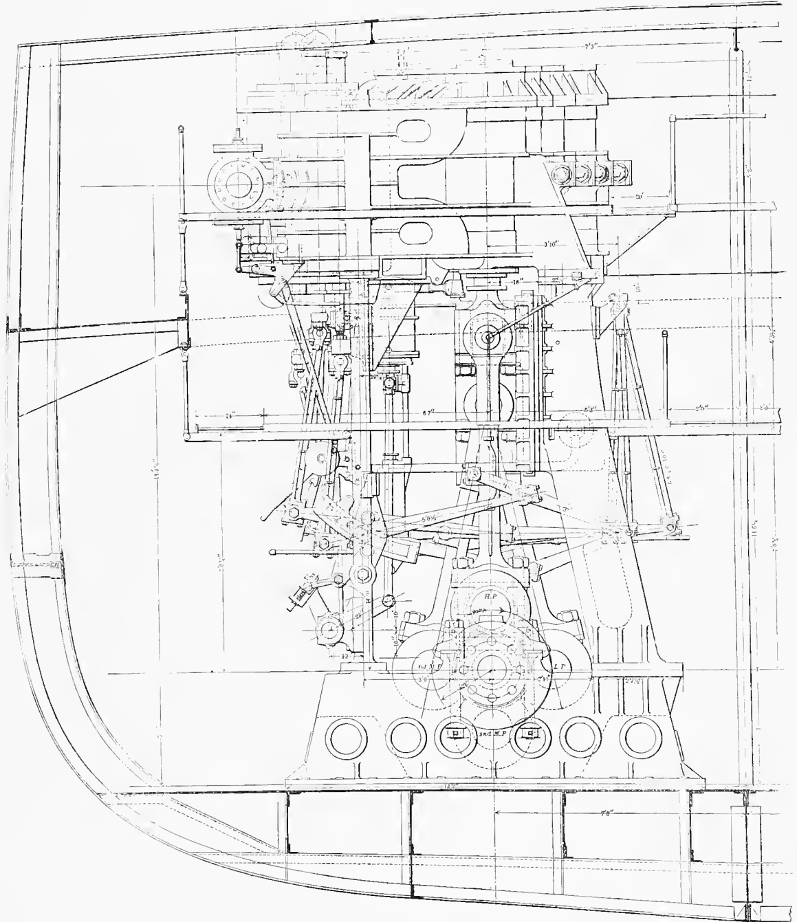
ENGINE OF TWIN-SCREW STEAMER NORTH WEST.
